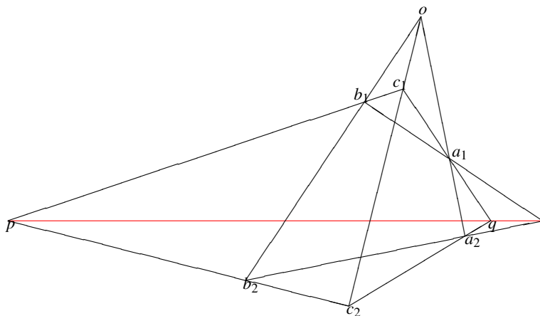
Figure 1.2: Desargues' Theorem
