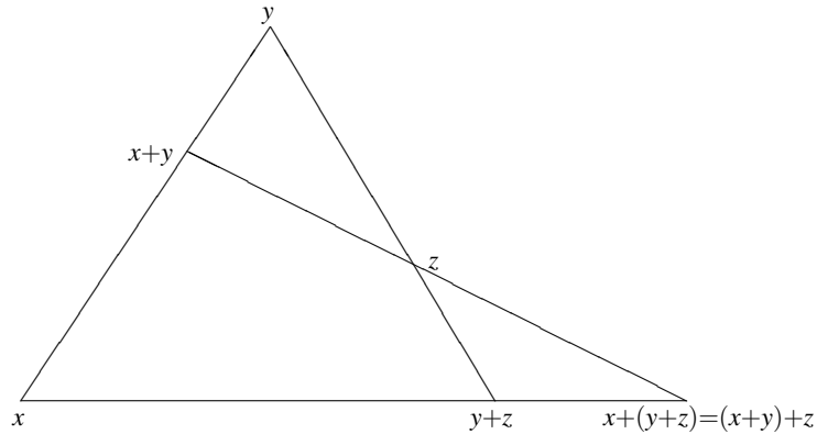
Figure 3.1: Veblen's Axiom
