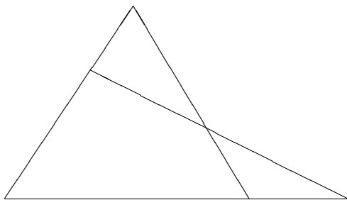
Figure 1.1: Veblen's Axiom
