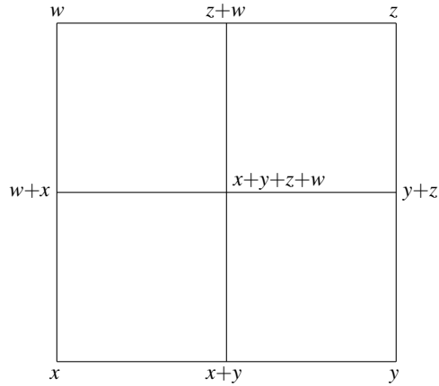
Figure 7.1: A grid
