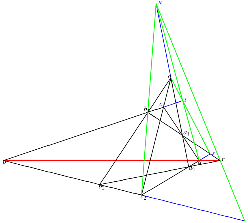
Figure 2.3: Pappus implies Desargues
