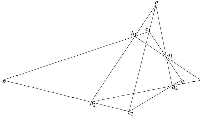
Figure 2.1: The Desargues configuration
